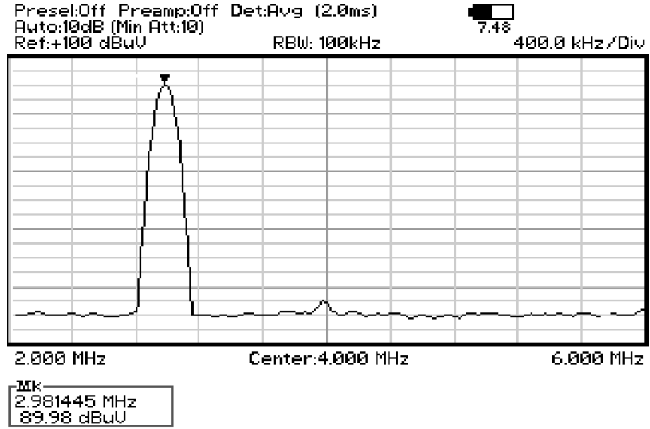
Fig. 3-3 Spectrum
