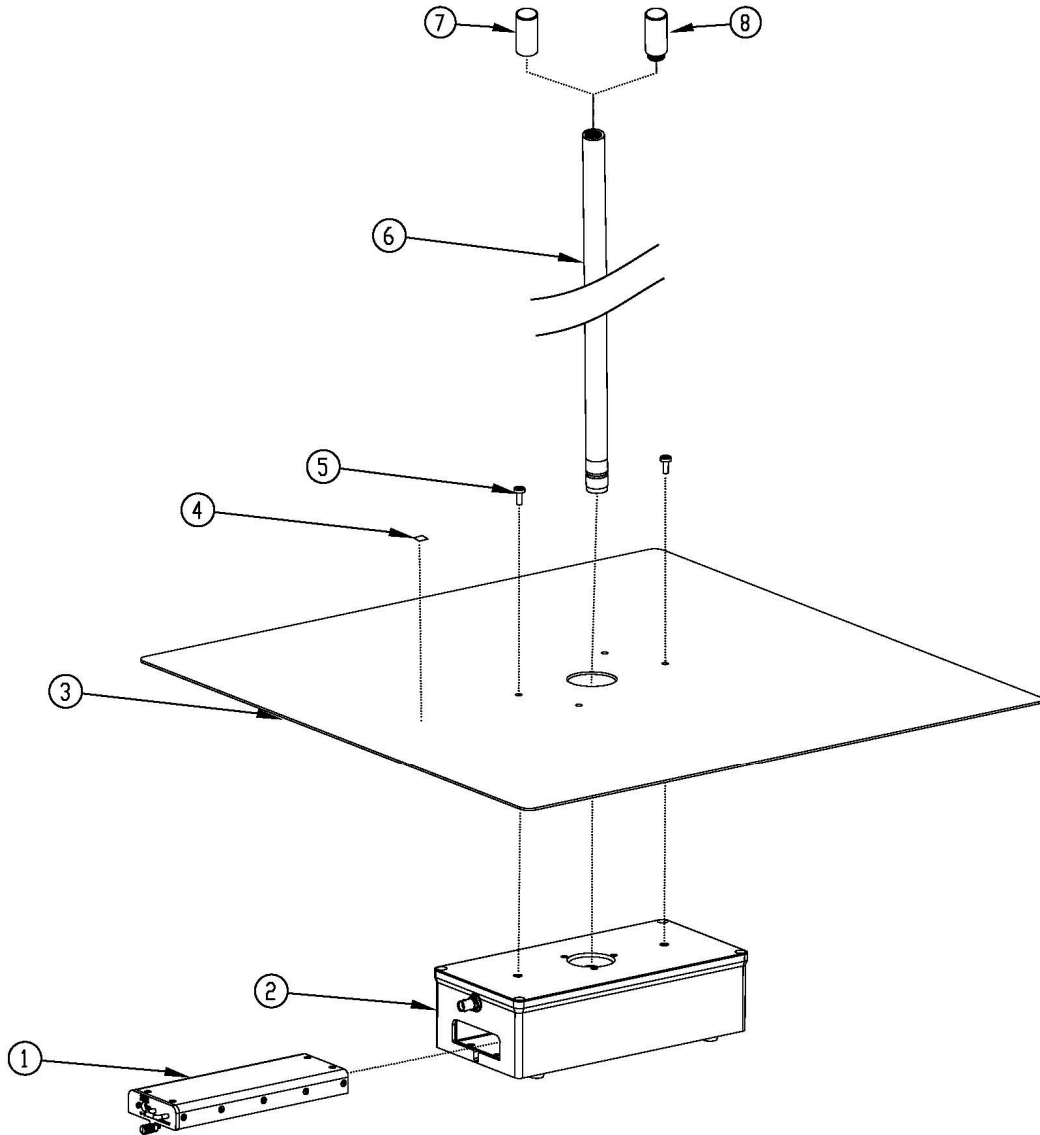
Fig. 2-1 Antenna parts and assembly
