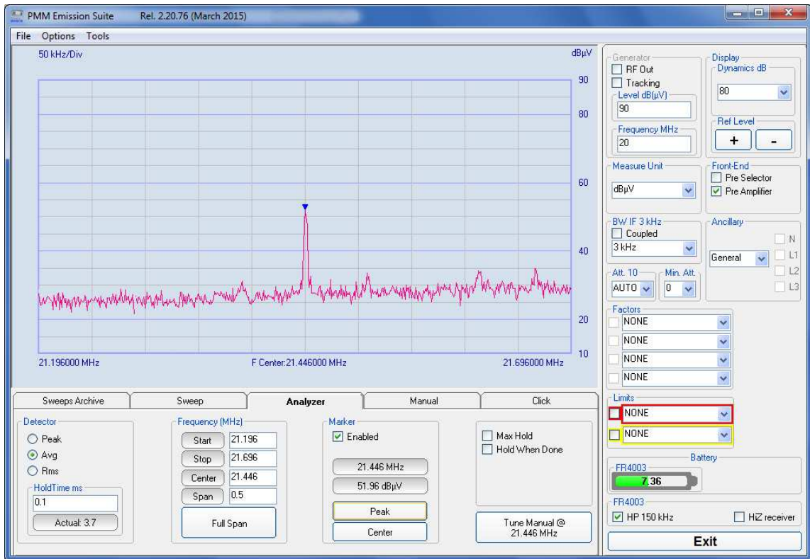
Fig. 4-3 Analyzer mode window
