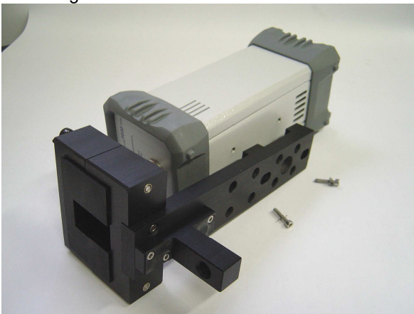
Mounting the PMM 9030/9060/9180 on the Antenna Holder
