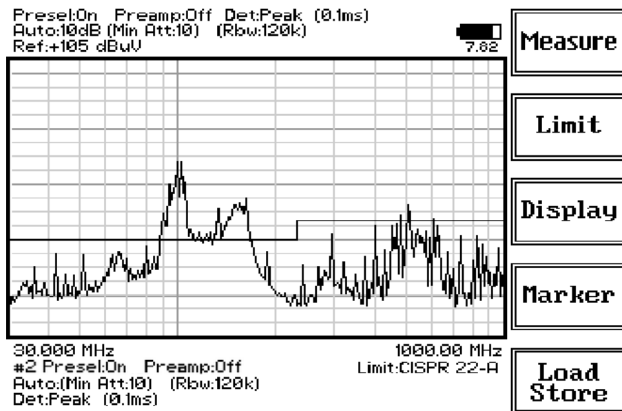
Fig. 11-9 Sweep
