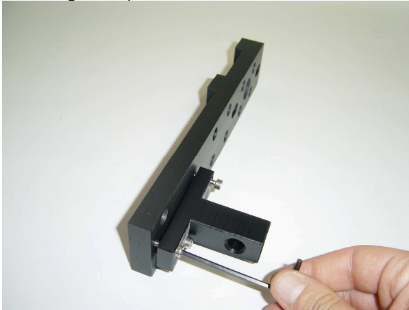
Mounting the tripod Joint
