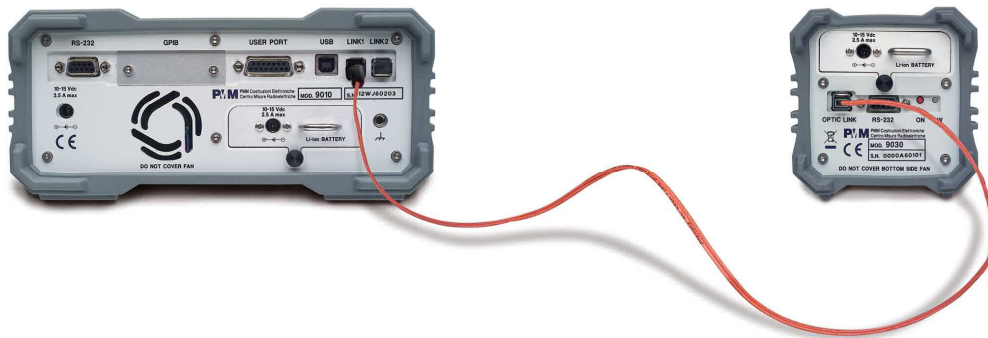
Fig. 11-5 PMM 9030/9060/9180 Fiber Optic Link to PMM 9010
