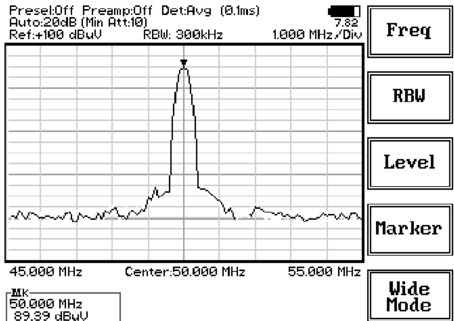
Fig. 11-8 Spectrum
