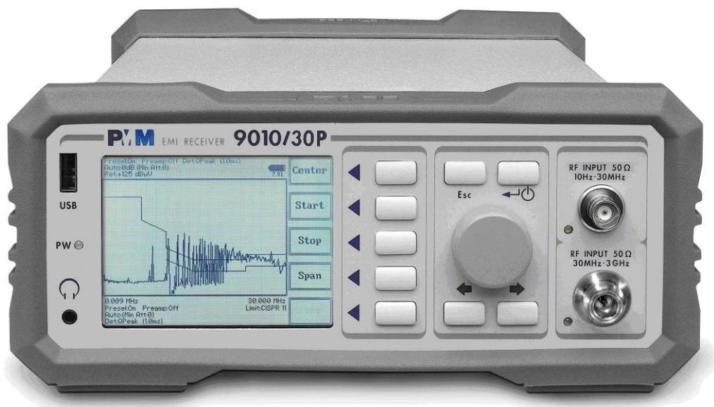
Fig. 9-4 Front Panel
