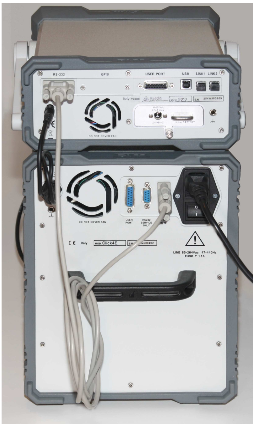
9010 and 9010 Click4E Option system rear view
