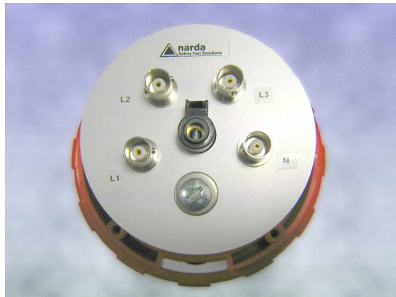
A-D-19 3-phase socket to BNC adapter. Model adequate to PMM L3-100 and higher (100 A sockets)
