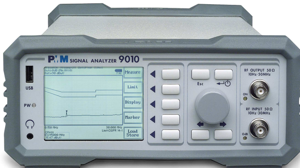
Fig. 1-1 Front Panel
