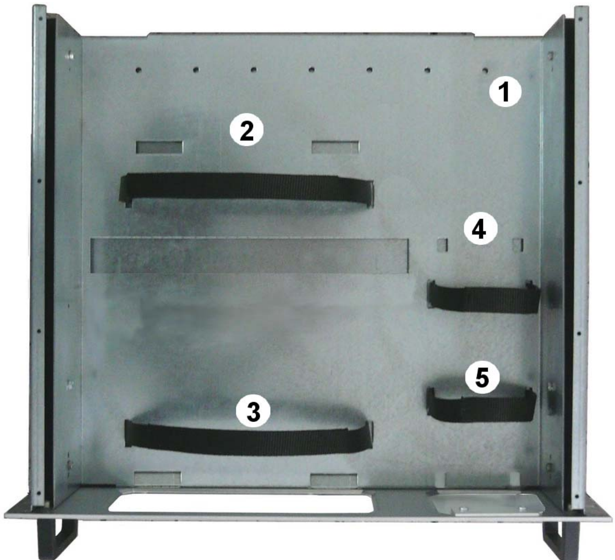
Fig. 8-2 Inside view
