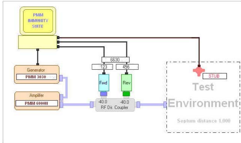
Fig. 6-1 Radiated immunity
