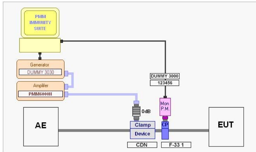
Fig. 6-2 Conducted immunity
